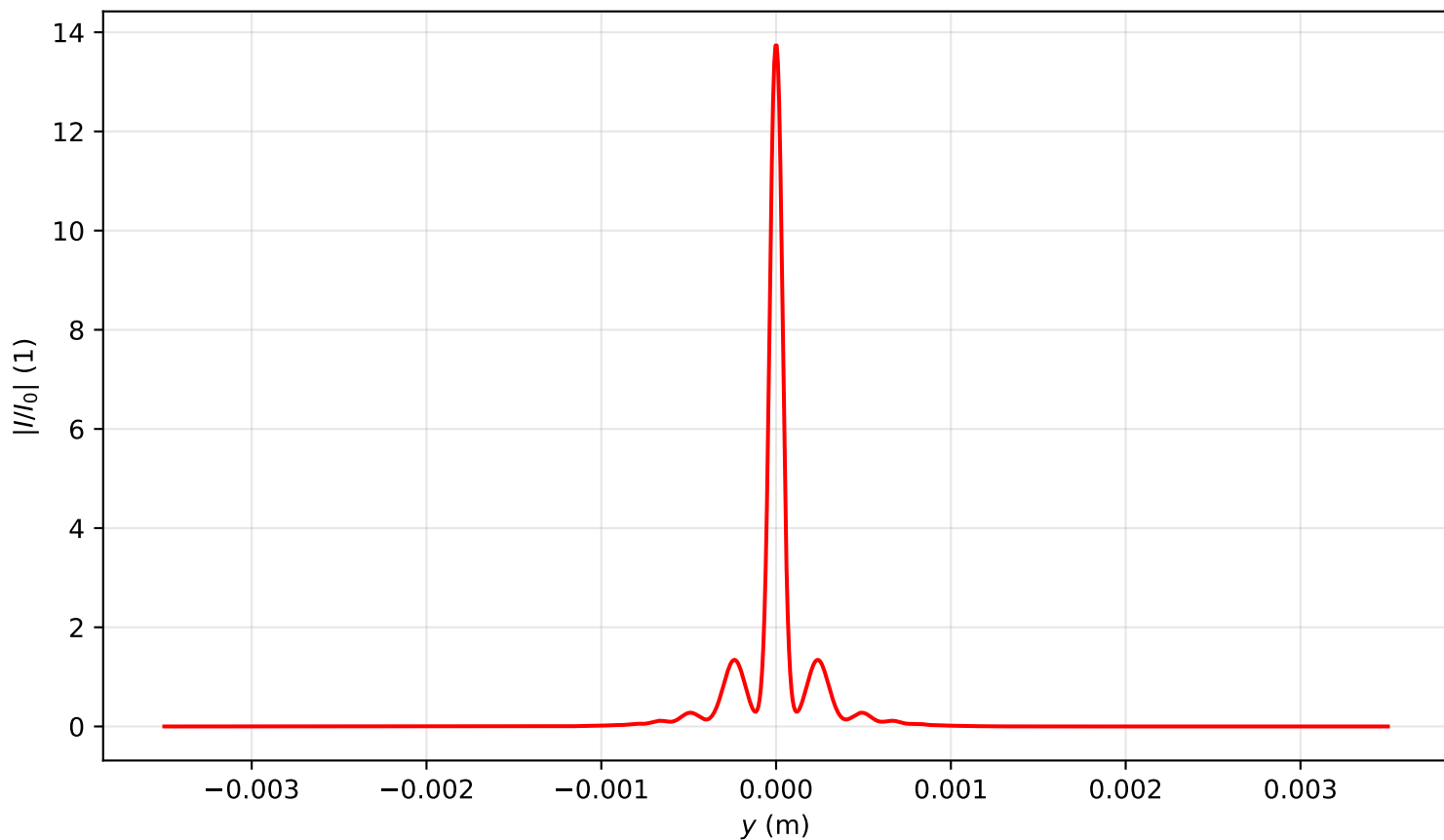
Intensity profile I(x = 0, y, z = 0.478)/I_0 , P_{in}=7.5P_{cr} , artificial time
